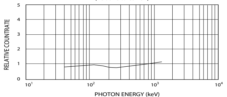
71313 ENERGY RESPONSE (Relative to Cs-137)
